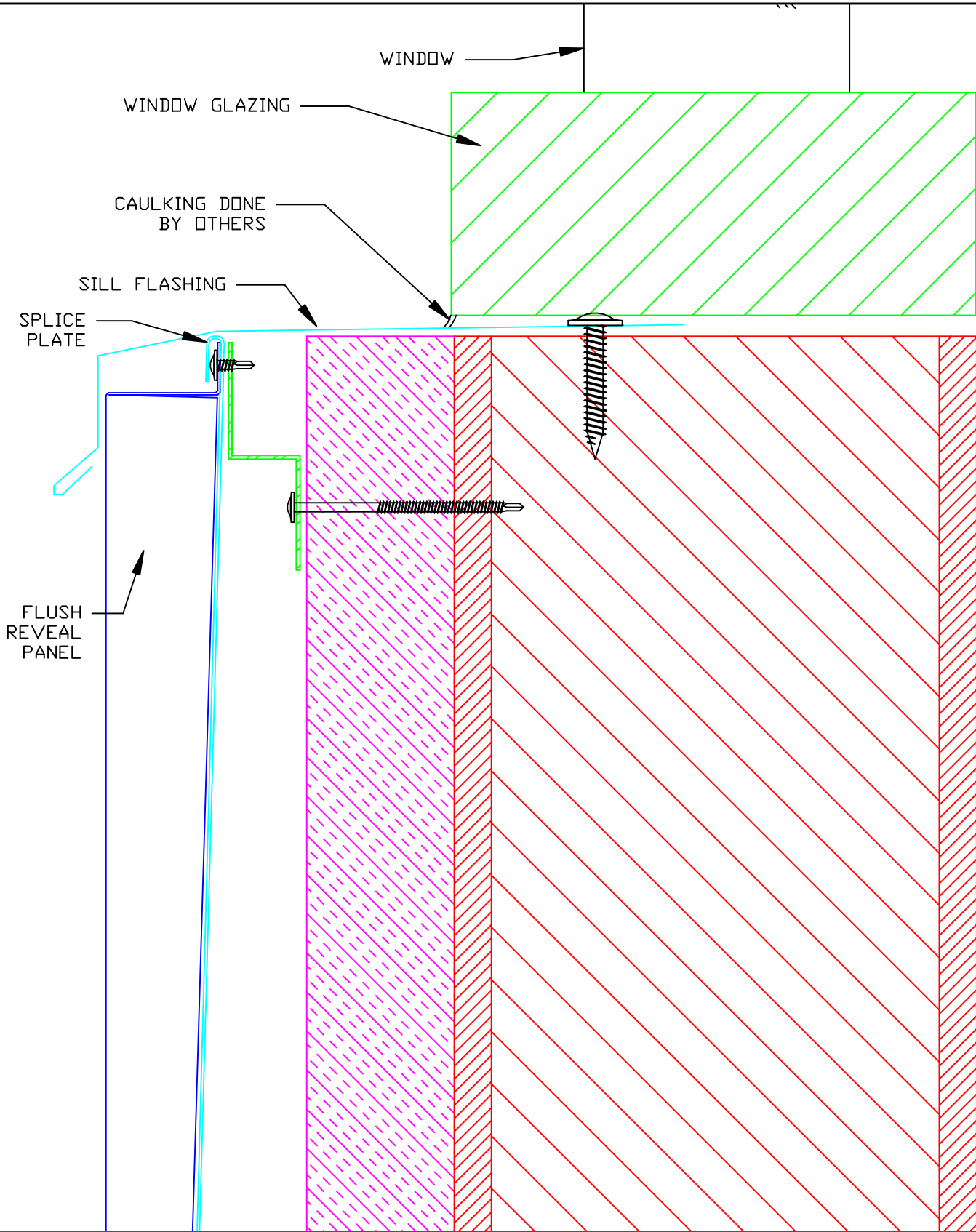
Horizontal Flush Reveal System - Window Sill
