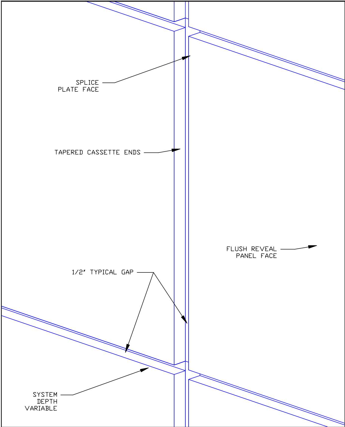
Horizontal Flush Reveal Cassette Joint System
