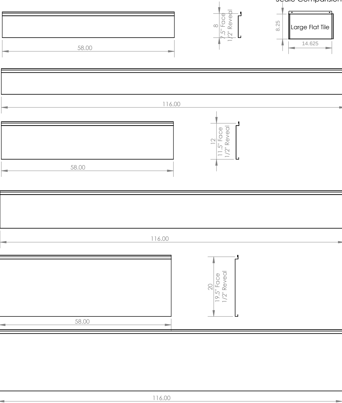
Horizontal Flush Reveal Cassette Joint Sizes
