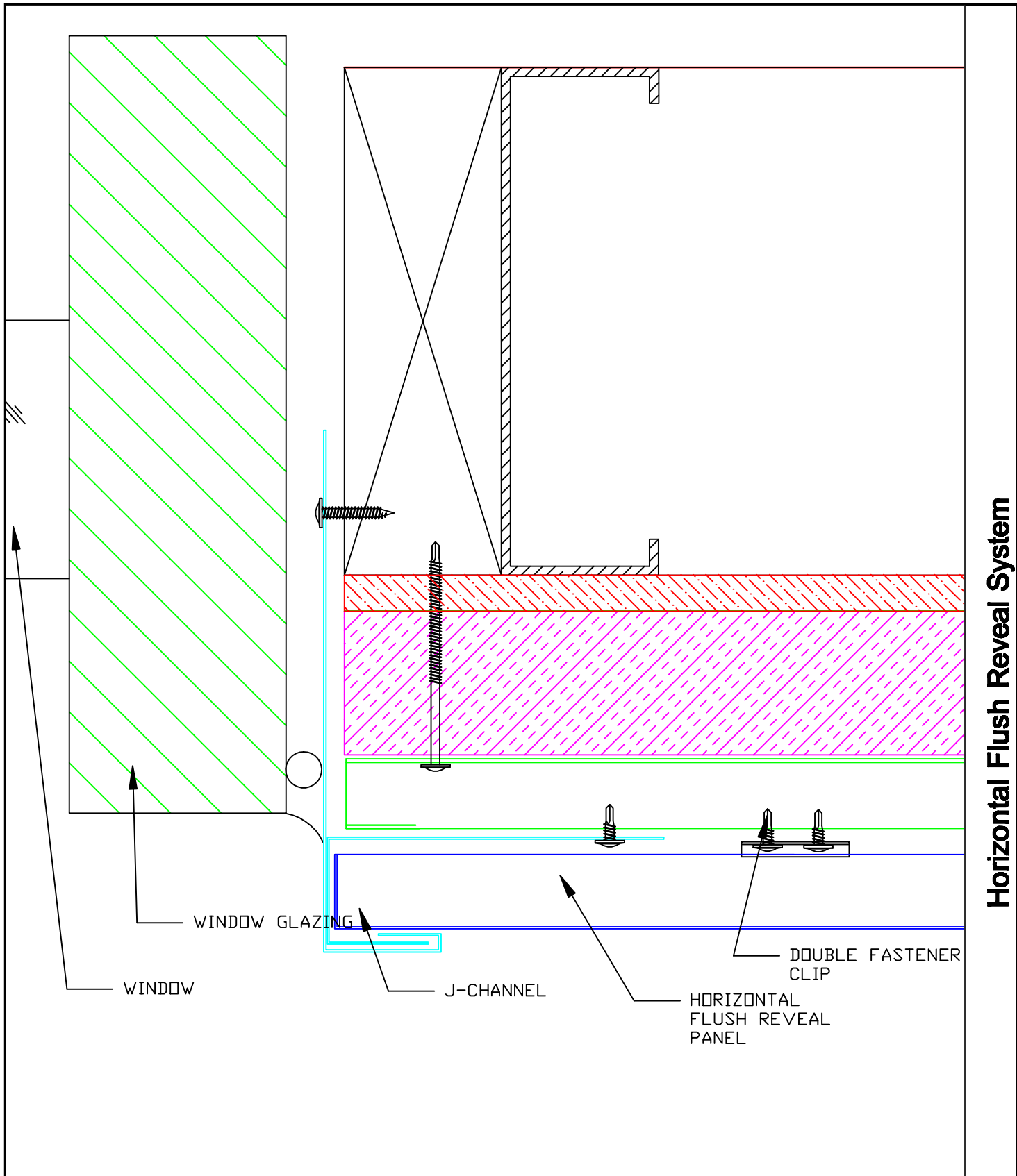
Horizontal Flush Reveal System - Window Jam
