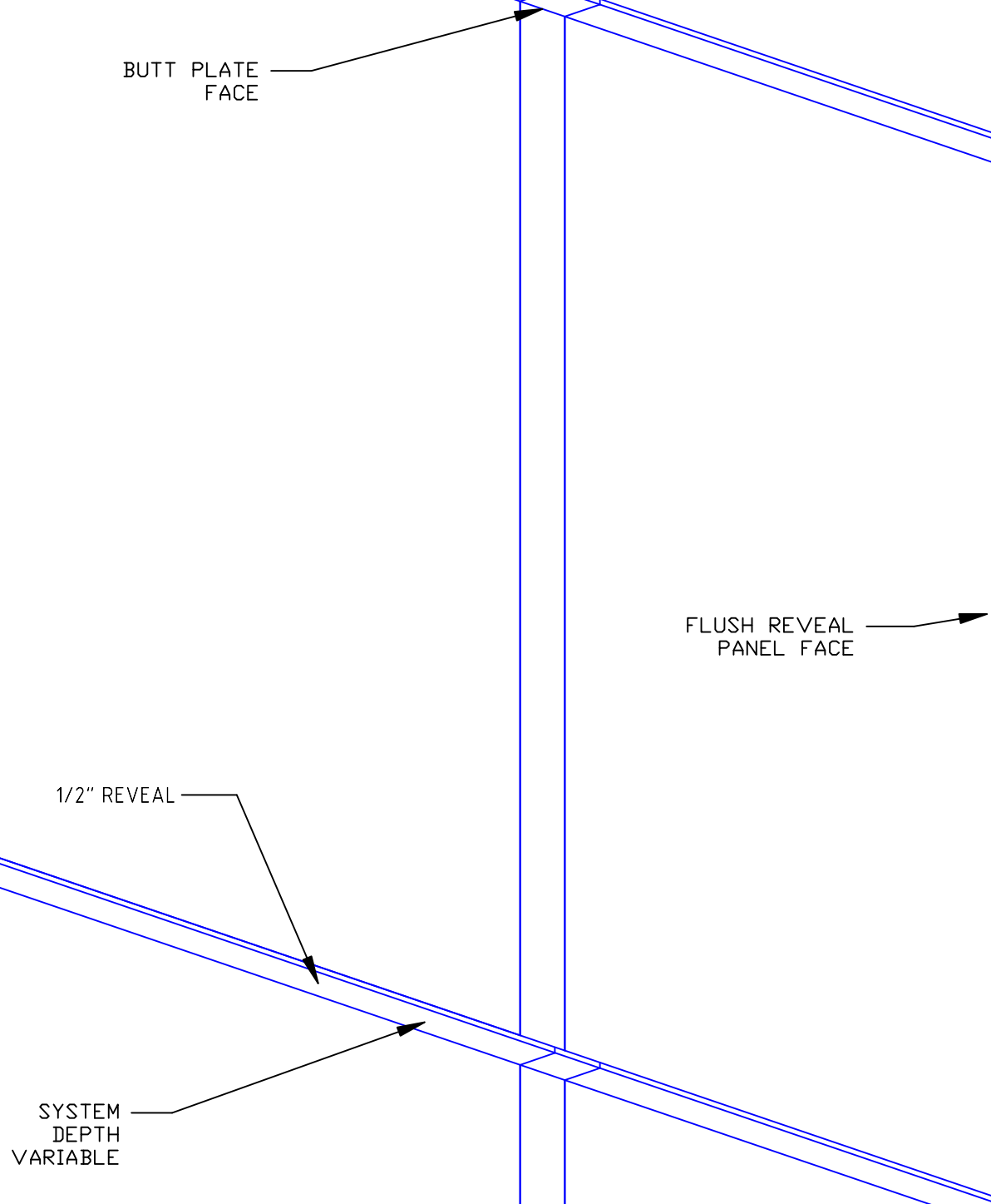
Horizontal Flush Reveal Butt Joint - System Details (Butt Plate)
