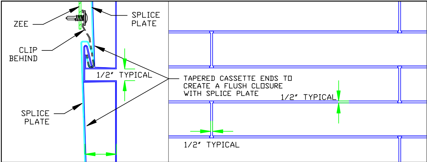
STANDARD SYSTEM DEPTH OF 1"
