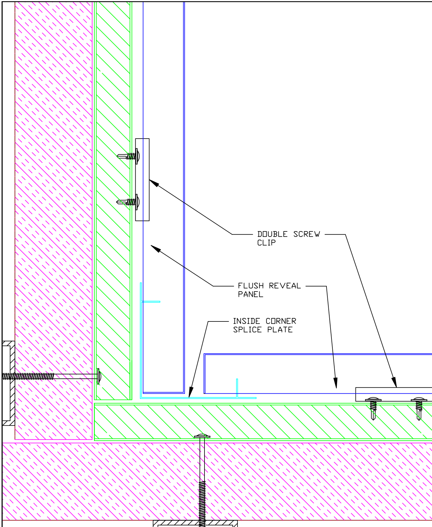
Horizontal Flush Reveal System - Inside Corner
