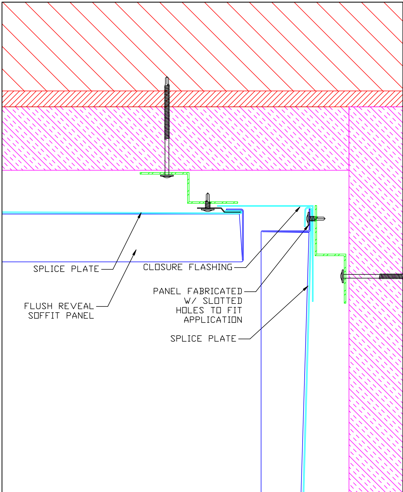
Horizontal Flush Reveal System - Soffit Return
