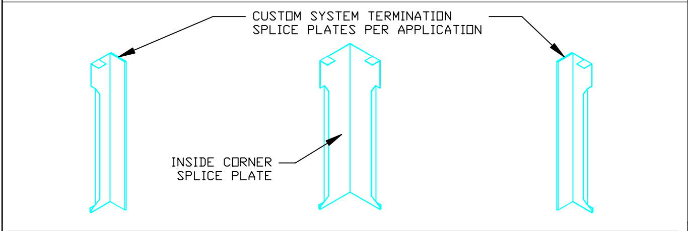
TYPICAL SPLICE PLATE
