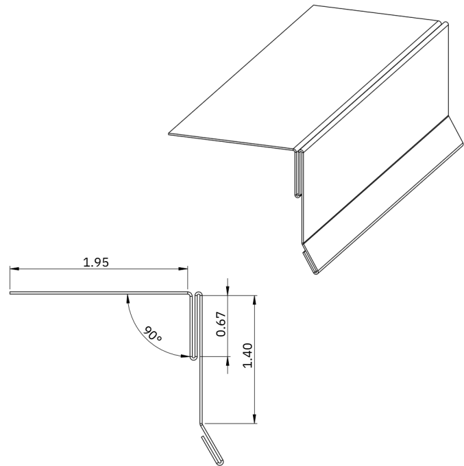
STARTER GABLE
