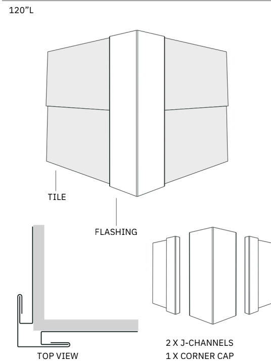
3 - PIECE
