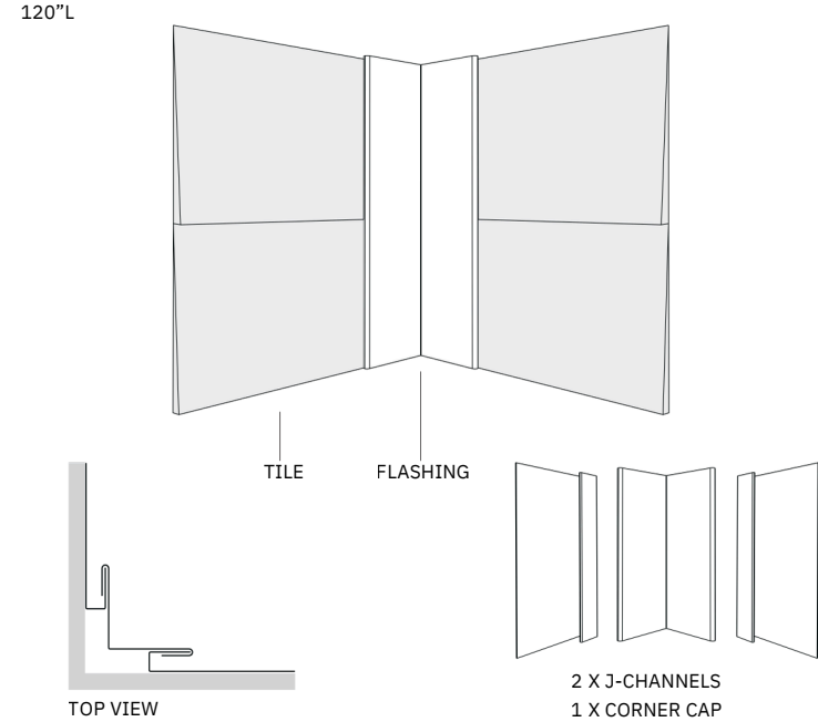
3 - PIECE
