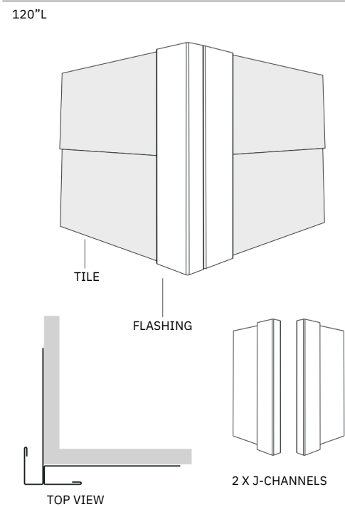
2 - PIECE
