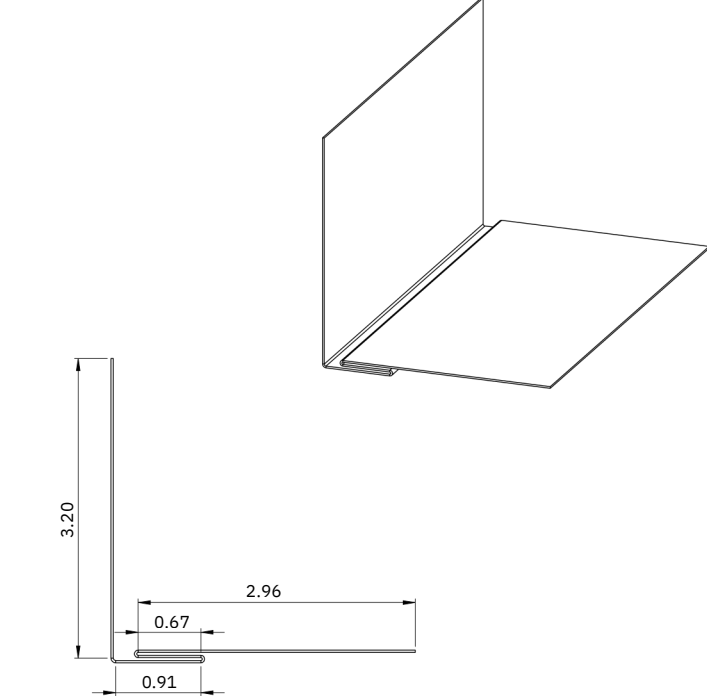
SIDE WALL
