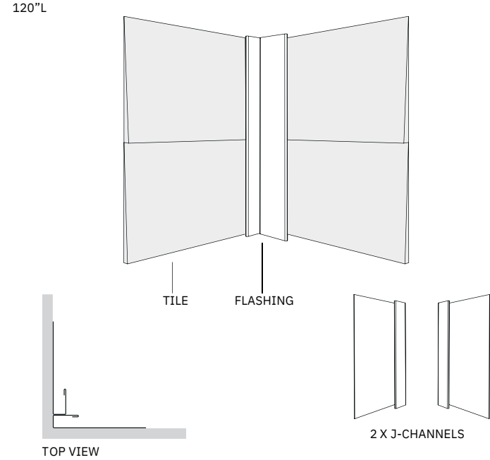
2 - PIECE
