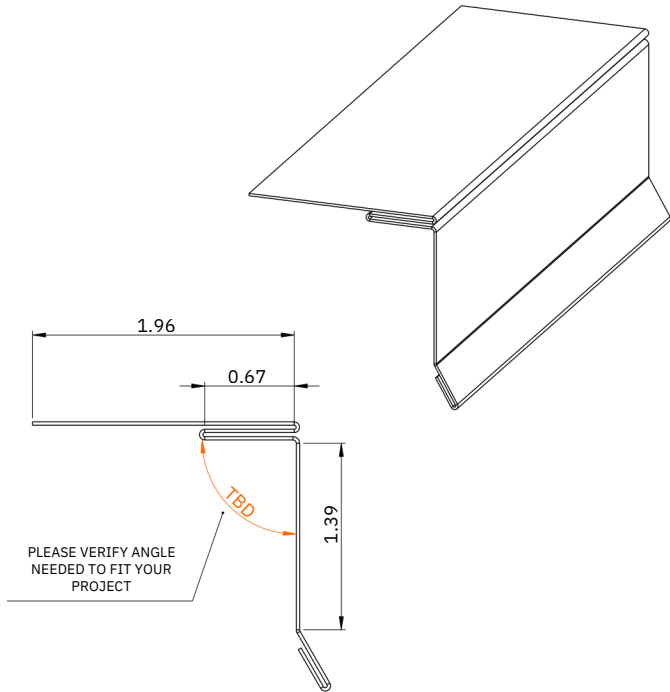
STARTER EAVE
